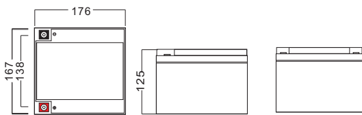
Terminal Dimensions
